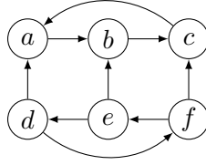
Figure 9: In this tournament, ME(T) = \{a, b, c\} whereas BA^\infty(T) = \{a, b, c, d, e, f\} . Omitted edges point downwards.
