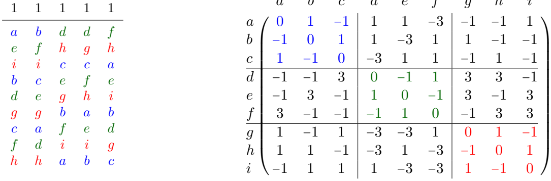
Figure 6: The preference profile R used in the proof of Theorem 4 is depicted on the left. The corresponding matrix of majority margins is illustrated on the right.
